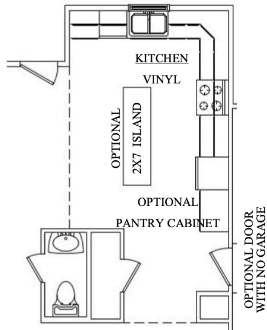
OPTIONAL KITCHEN #2
